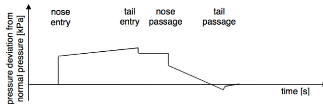
Fig. 4. Pressure deviation caused by a train along the tunnel(3)(Reinke, 2011)
