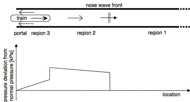
Fig. 2. Pressure deviation caused by a train along the tunnel(1)(Reinke, 2011)
