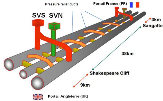
Fig. 1. Pressure relief ducts installed in the Channel tunnel
